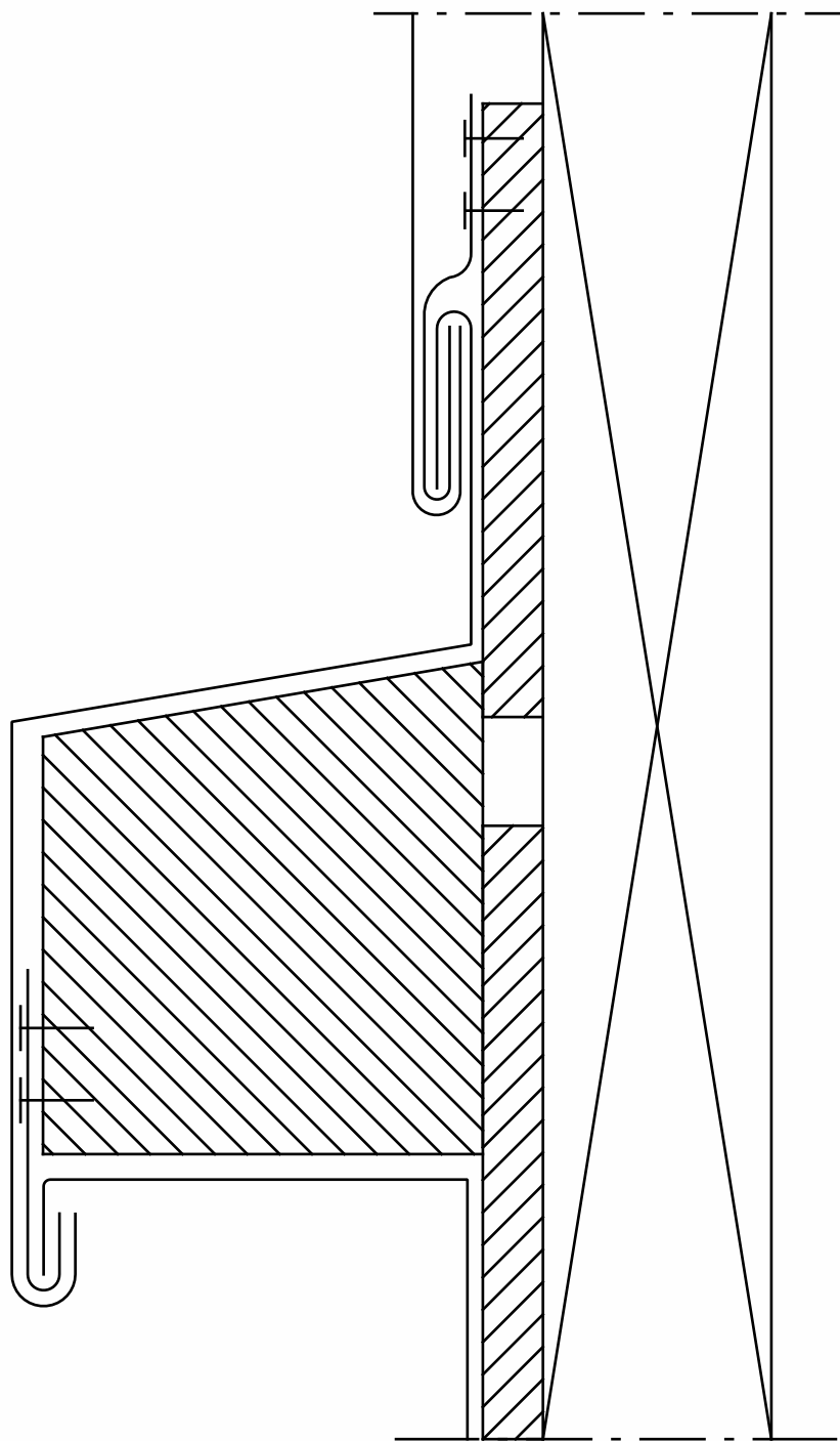
Vertical section
