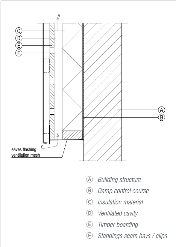
Figure 6.1.7 Eaves connection
