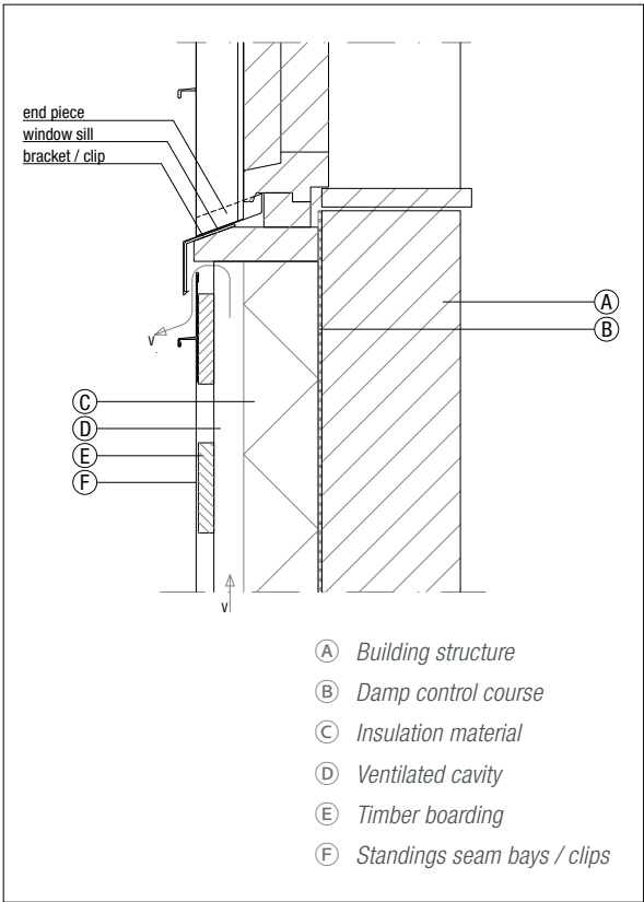
Figure 6.1.15 Window sill
