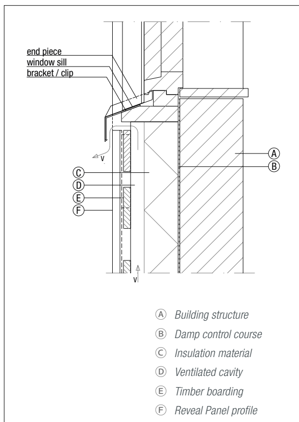
Figure 6.4.7 Window sill
