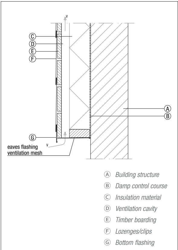
Figure 6.3.9 Eaves connection
