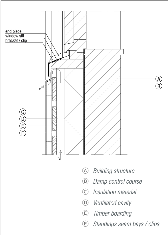
Figure 6.1.8 Window sill
