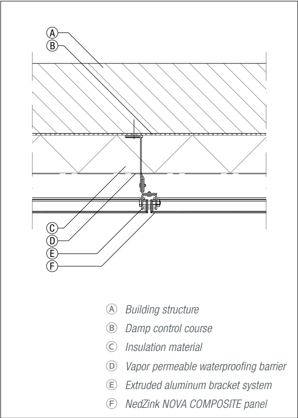
Figure 6.5.4 Vertical joint
