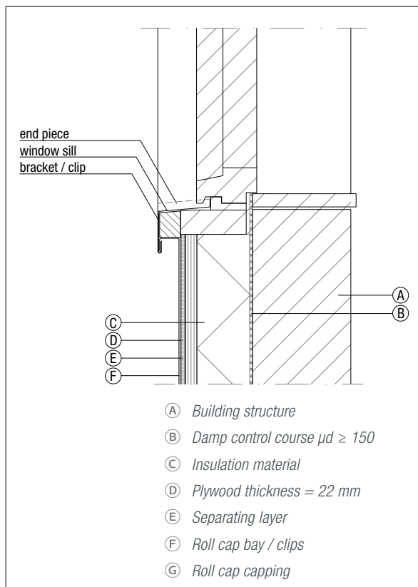
Figure 6.2.31 Window sill
