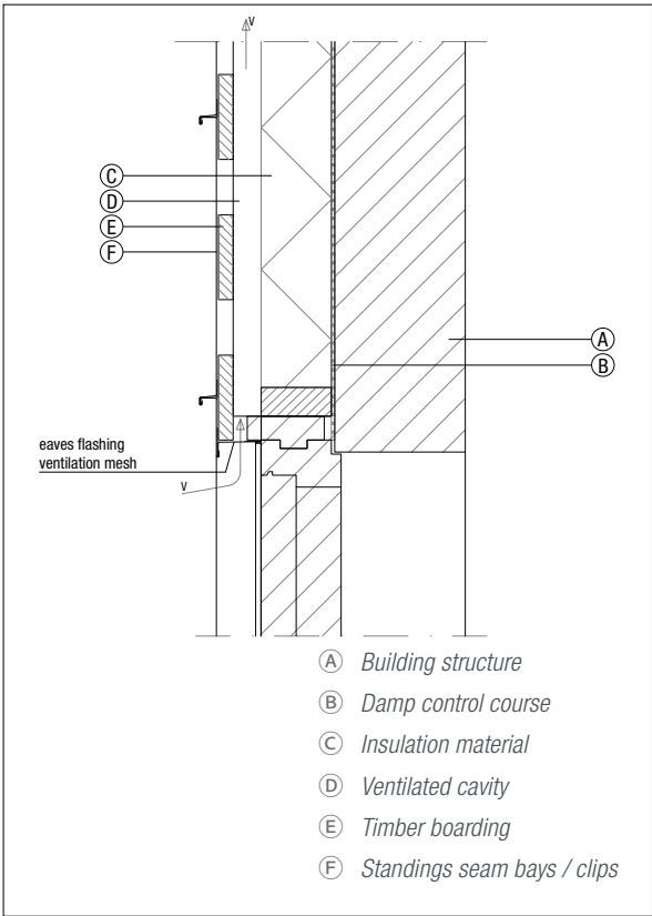
Figure 6.1.16 Window head
