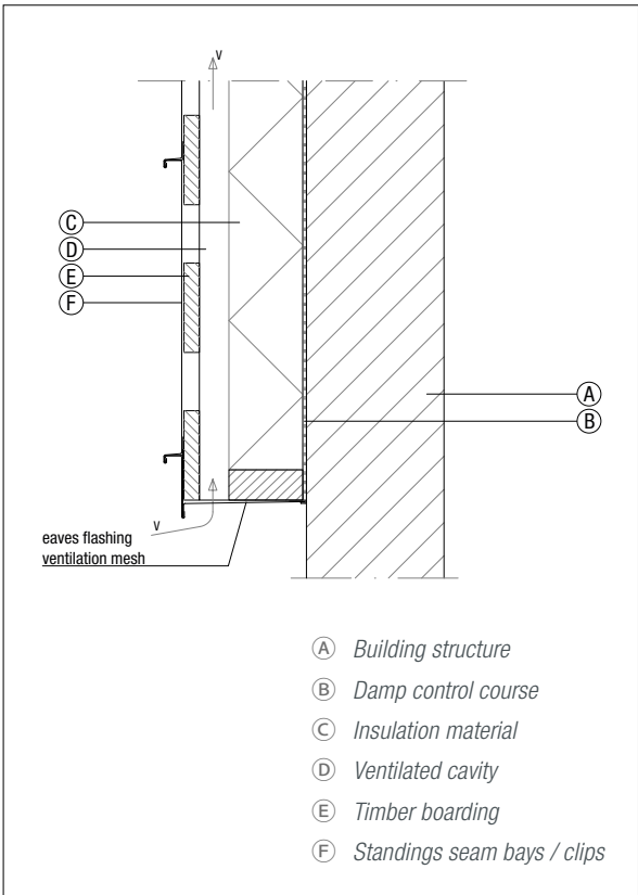
Figure 6.1.14 Eaves connection
