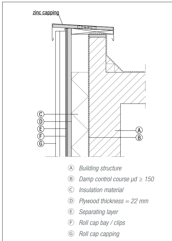
Figure 6.2.22 Ridge connection
