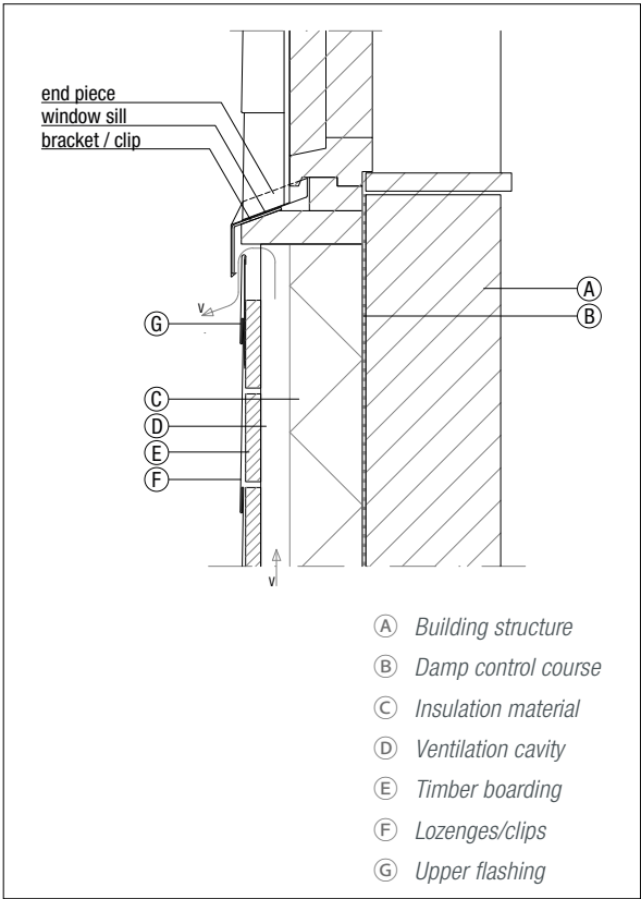
Figure 6.3.10 Window sill
