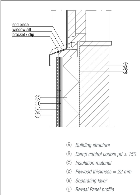
Figure 6.4.22 Window sill
