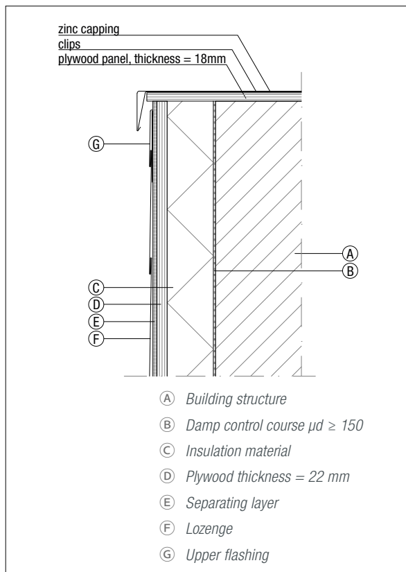
Figure 6.3.16 Ridge connection
