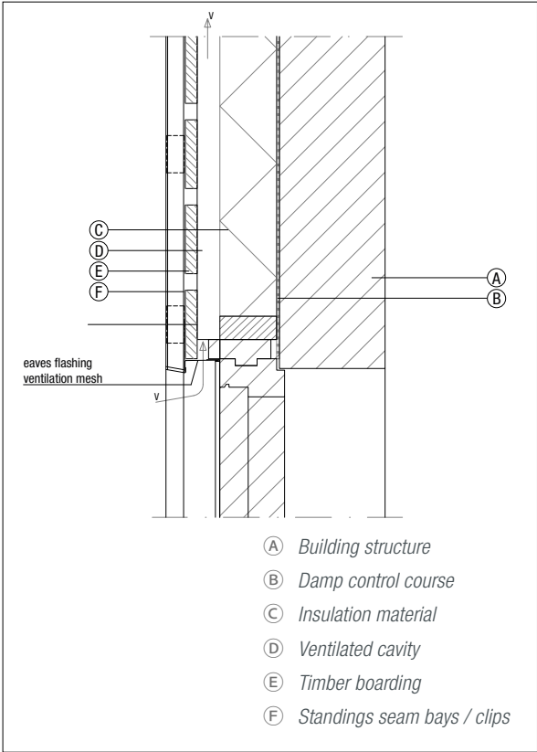
Figure 6.1.9 Window head
