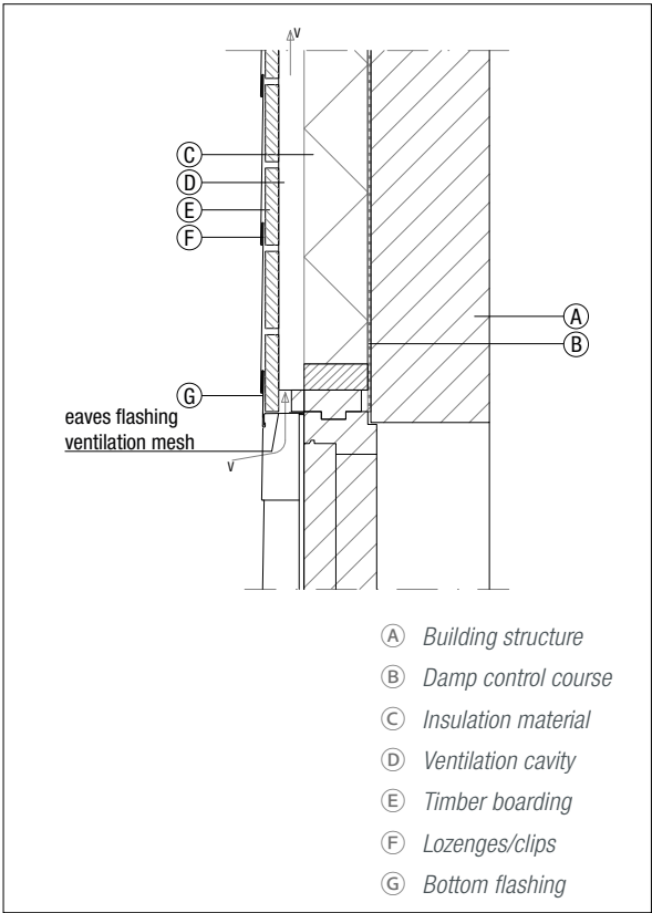
Figure 6.3.11 Window head
