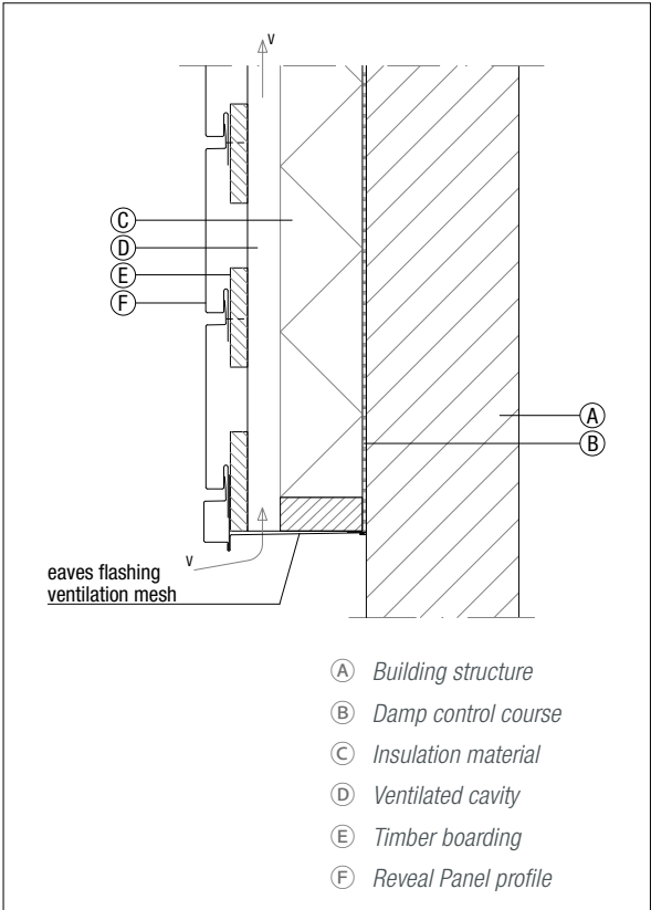
Figure 6.4.13 Eaves connection
