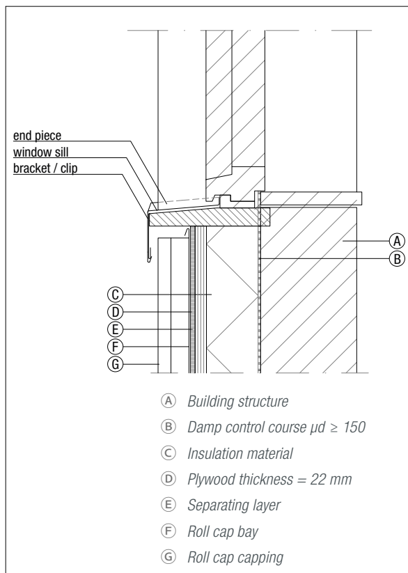
Figure 6.2.24 Window sill
