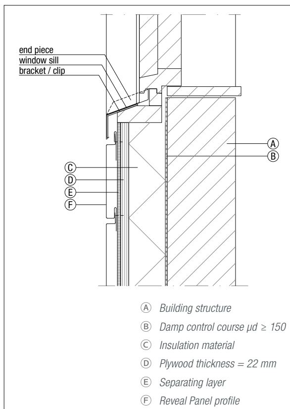
Figure 6.4.29 Window sill
