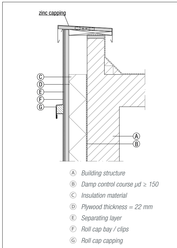
Figure 6.2.29 Ridge connection
