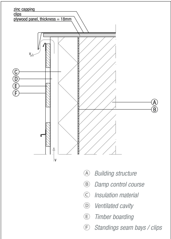
Figure 6.1.13 Ridge connection
