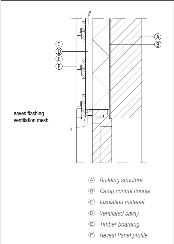
Figure 6.4.15 Window head
