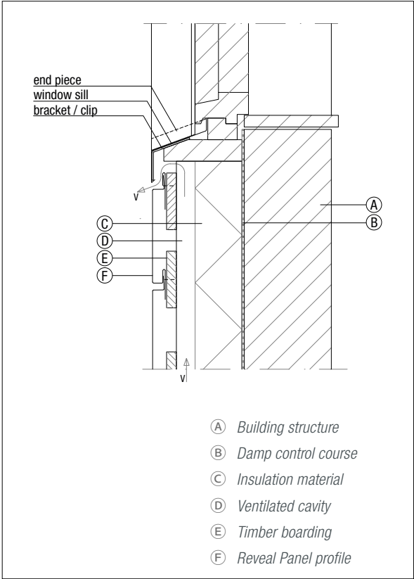
Figure 6.4.14 Window sill
