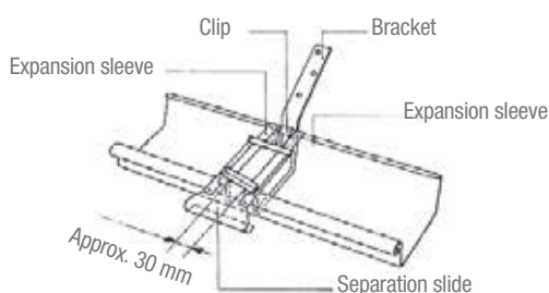
Figure 3.6 Zinc expansion device installed
