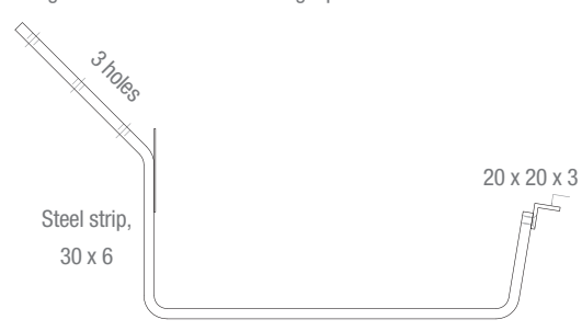
Figure 4 Bracket with steel angle profile
