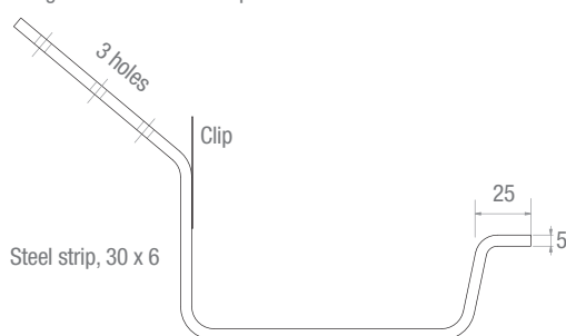
Figure 3 Bracket with lip
