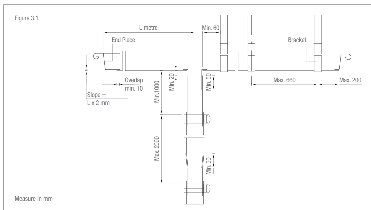
Longitudinal-section of the roof gutter in the bracket.
